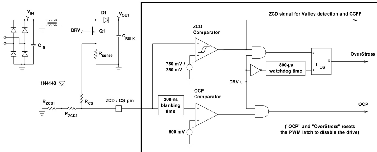
Figure 70. Current Sense and Zero Current Detection Blocks
