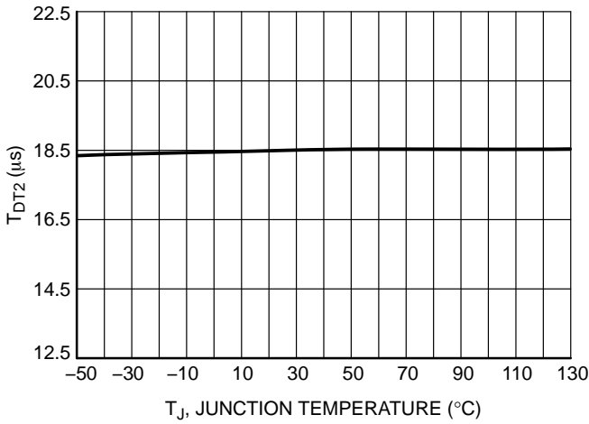
Figure 12. Dead-time, V_{\text{FFcontrol}} = 1.75 \text{ V} vs. Temperature
