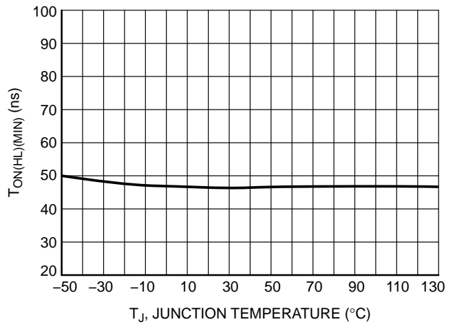
Figure 43. Minimum On Time @ V SENSE = 2.8 V vs. Temperature
