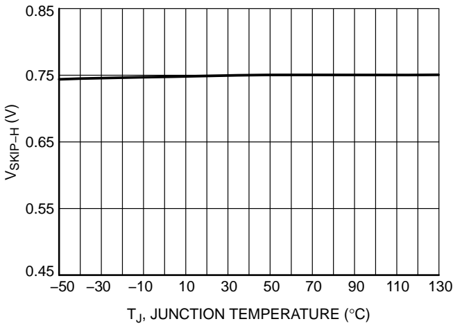
Figure 14. FFcontrol Pin Skip Level ( V_{\text{FFcontrol}} Rising) vs. Temperature
