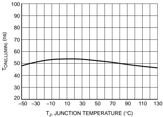
Figure 42. Minimum On Time @ V SENSE = 1.4 V vs. Temperature
