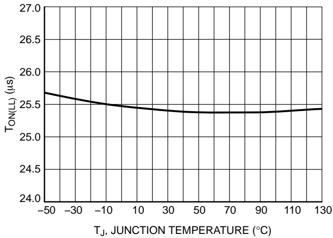
Figure 40. Maximum On Time @ V SENSE = 1.4 V vs. Temperature
