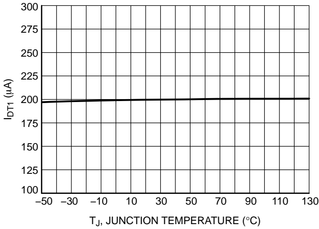
Figure 10. FFcontrol Pin Current, V_{\text{SENSE}} = 1.4 \text{ V} and V_{\text{CONTROL}} Maximum vs. Temperature
