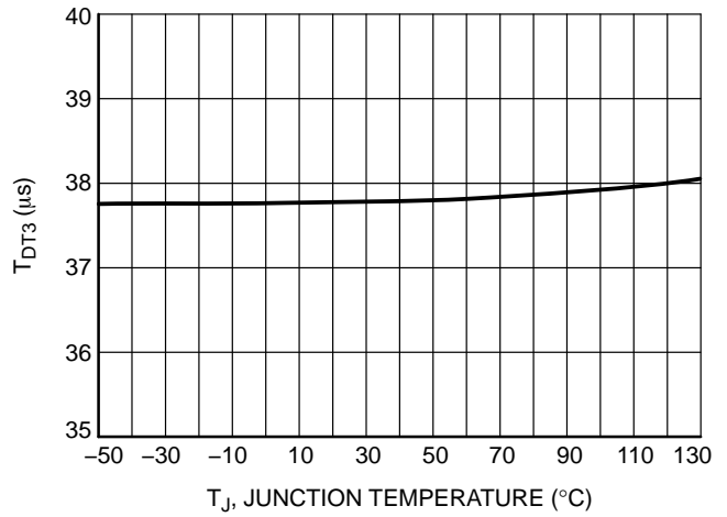
Figure 13. Dead-time, V_{\text{FFcontrol}} = 1.00 \text{ V} vs. Temperature
