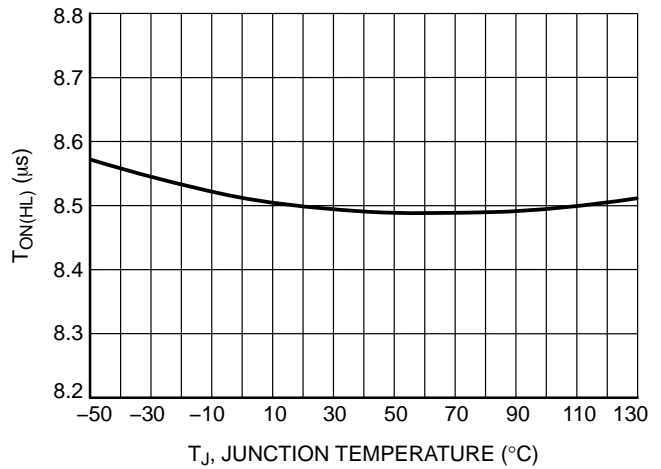
Figure 41. Maximum On Time @ V SENSE = 2.8 V vs. Temperature
