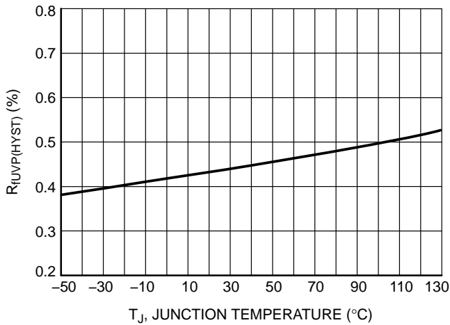
Figure 50. Ratio (UVP Hysteresis) over V REF vs. Temperature
