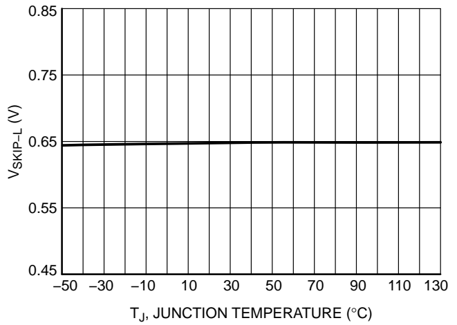
Figure 15. FFcontrol Pin Skip Level ( V_{\text{FFcontrol}} Falling) vs. Temperature
