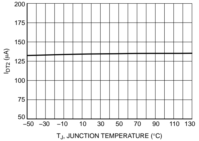
Figure 11. FFcontrol Pin Current, V_{\text{SENSE}} = 2.8 \text{ V} and V_{\text{CONTROL}} Maximum vs. Temperature
